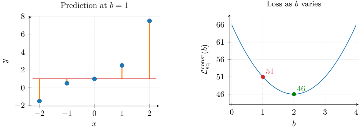
Figure 5: Left: the input axis is x , and the constant prediction b = 1 gives squared loss 51. Right: the horizontal axis is the parameter b , and the curve is \mathcal{L}_{\text{sq}}^{\text{const}}(b) = 5b^2 - 20b + 66 . Its minimum is 46, attained at b = 2 .
